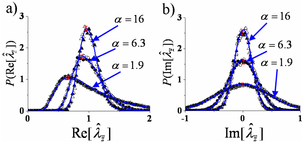
Fig. 5.1: PDFs for the real (a) and imaginary (b) parts of the grouped eigenvalues of the normalized cavity impedance \hat{\lambda}_z (hollow stars : Loss-Case 0; hollow circles : Loss-Case 1; hollow triangles : Loss-Case 2) in the frequency range of 10.5-12 GHz. The PDFs for the real (a) and imaginary (b) parts of the grouped eigenvalues of the normalized cavity admittance \hat{\lambda}_y (solid stars : Loss-Case 0; solid circles : Loss-Case 1; solid triangles : Loss-Case 2) in the frequency range of 10.5-12 GHz are also shown. The red error bars indicate the typical statistical binning error of the data. Also shown are the single parameter, simultaneous fits for both impedance and
