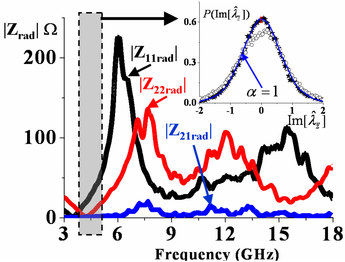
Fig. 5.5: Magnitude of the elements of the measured radiation impedance matrix are shown as a function of frequency from 3 to 18 GHz for the setup in Fig.3.3. Inset: PDF of \text{Im}[\hat{\lambda}_z] for the Loss Case 0 cavity in the frequency range 4-5 GHz, which is obtained by considering the full 2x2 radiation impedance matrix (stars) and by considering only the contribution of the diagonal elements of the radiation impedance matrix (circles). The blue solid line is the Random Matrix Theory numerical prediction for \alpha=1 which is obtained from the variance of the data represented by the stars.
