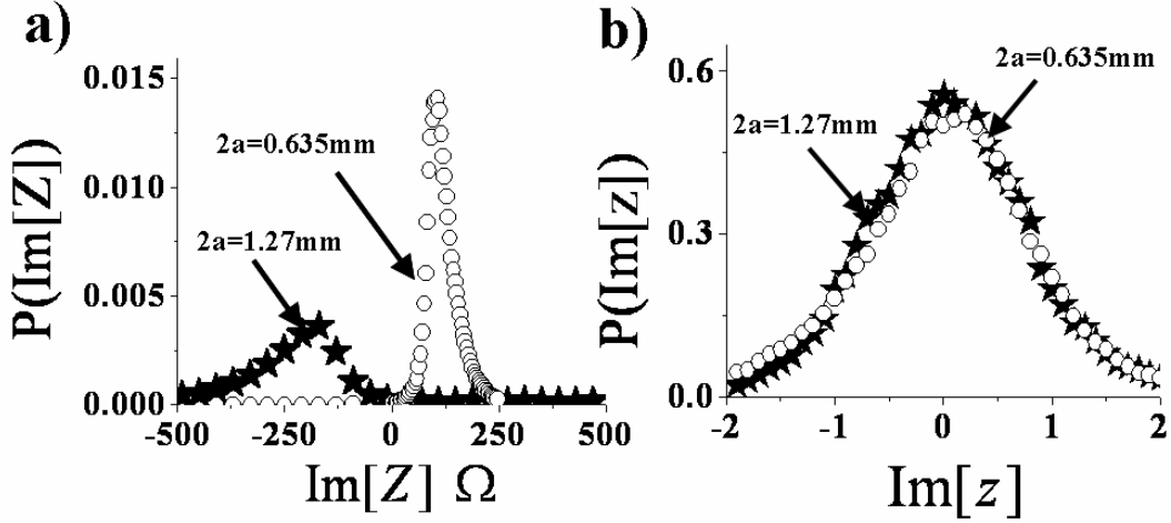
Fig.4.3: (a) shows the PDFs of the imaginary part of cavity impedance ( \text{Im}[Z] ) for two different antenna diameters, 2a=0.635\text{mm} (circles) and 2a=1.27\text{mm} (stars), from 9 GHz to 9.6 GHz. (b) The two curves in (a) scale together after using the prescription of [25] for the imaginary normalized cavity impedance ( \text{Im}[z] ).
